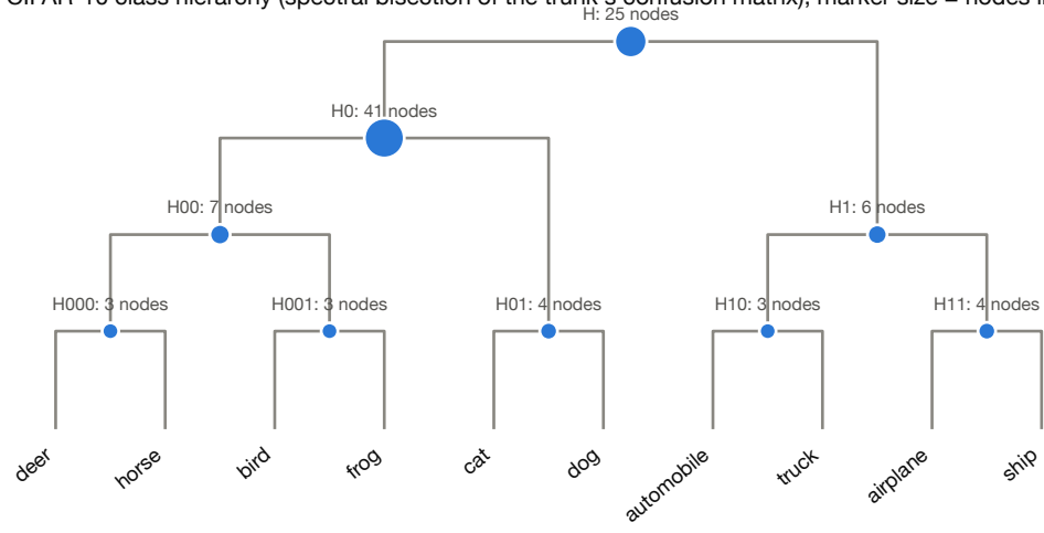
CIFAR-10 class hierarchy (spectral bisection of the trunk's confusion matrix); marker size = nodes in that split's tree
