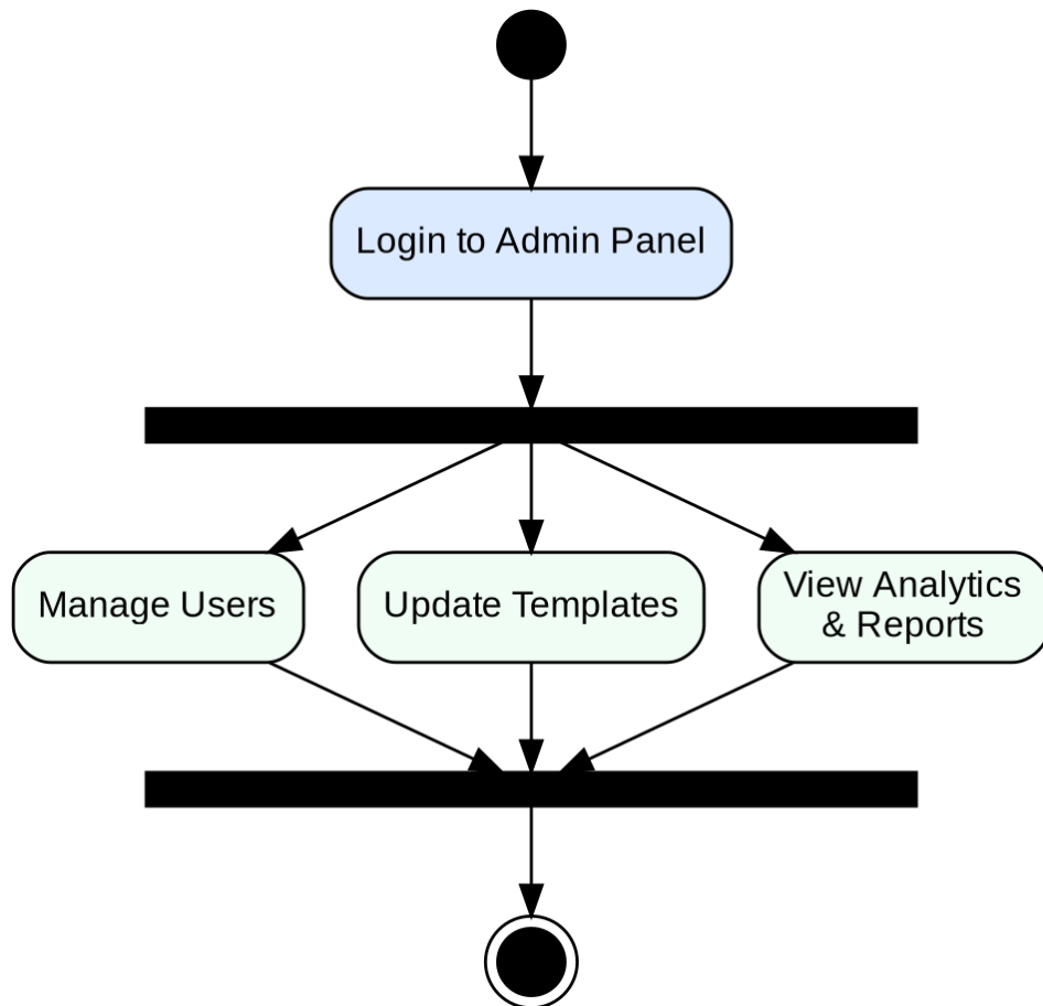
Figure 3.7: Activity Diagram for Admin
