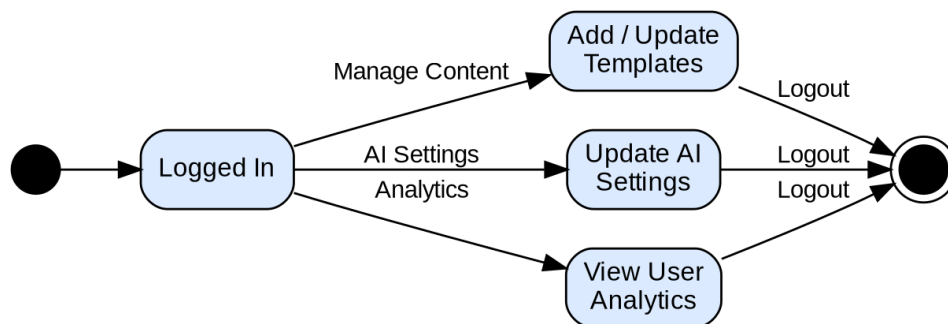
Figure 3.9: State Diagram for Admin
