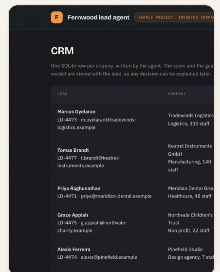
Scored CRM
