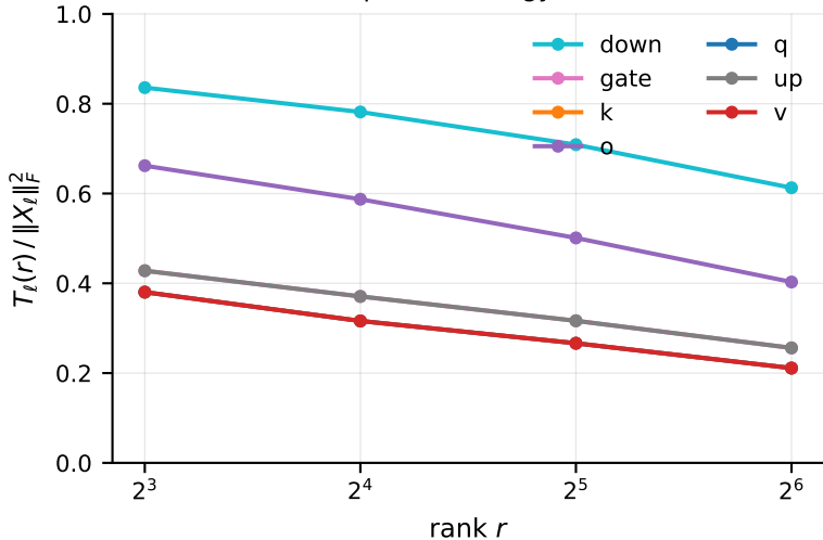
Qwen3-0.6B: spectral energy left after rank r
