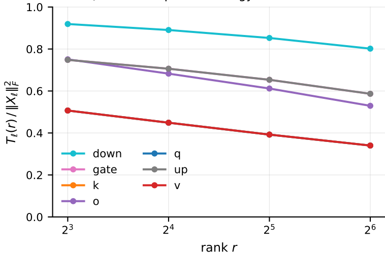
Qwen3-8B: spectral energy left after rank r
