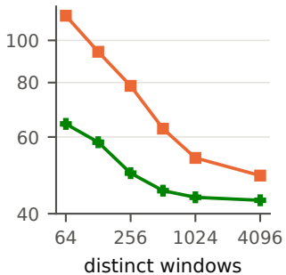
WikiText-2 perplexity
