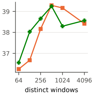
mean accuracy (%)
