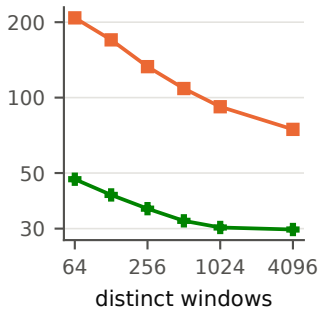
SlimPajama perplexity
