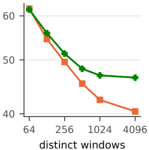
C4 perplexity
