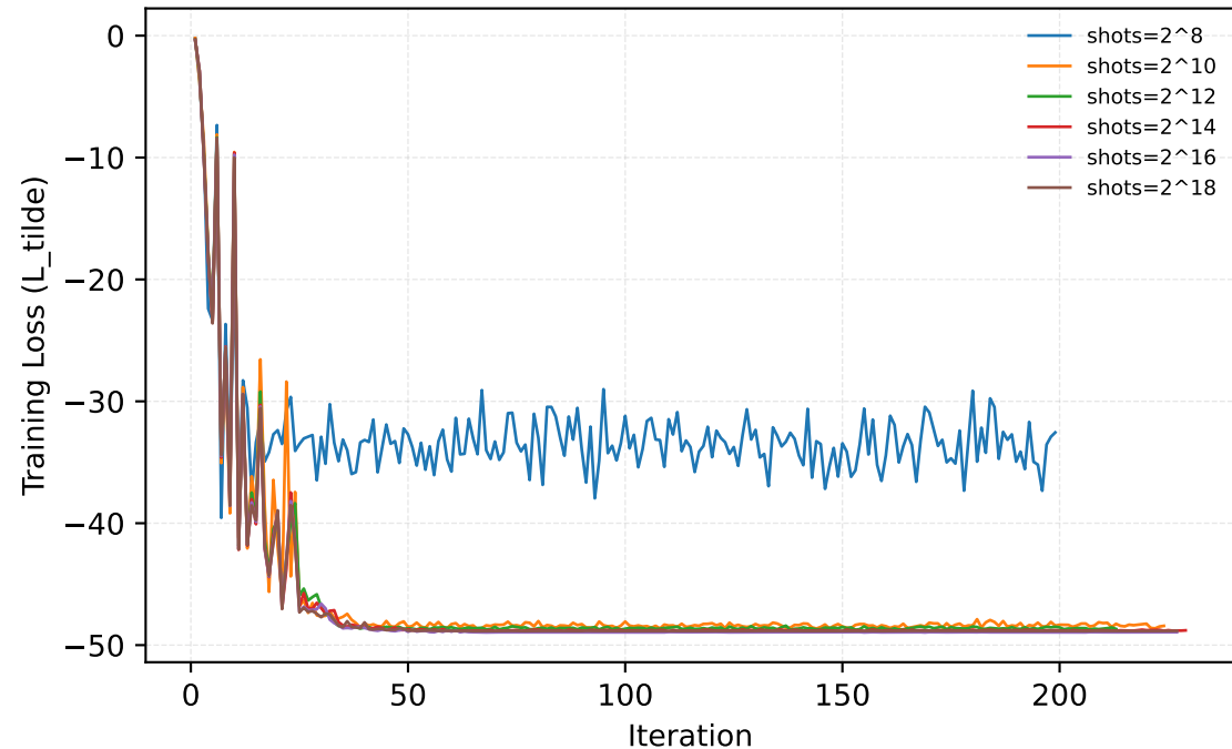
Training Convergence over Shot Budgets
