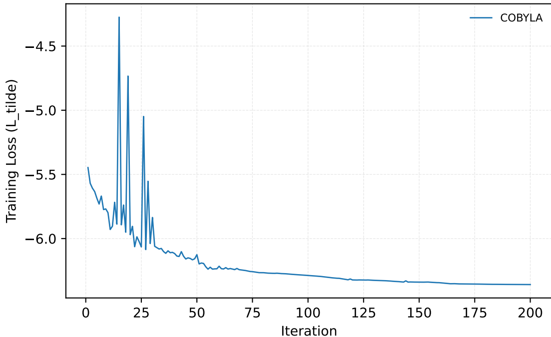
VQBR Training Convergence (COBYLA)
