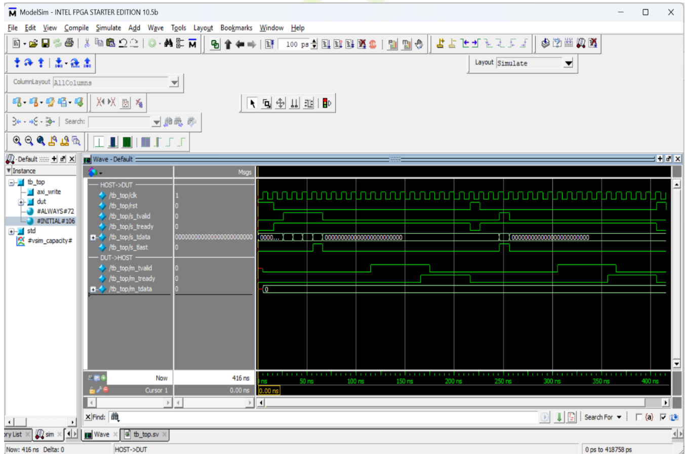
Fig 4 Simulation Waveform
