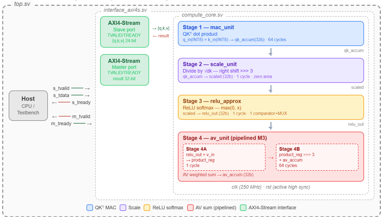
Fig. 2 — Full system block diagram showing host, AXI4-Stream interface (interface_axi4s.sv), and 4-stage compute core (compute_core.sv) with pipelined av_unit. Total pipeline latency: 195 cycles at 250 MHz.
