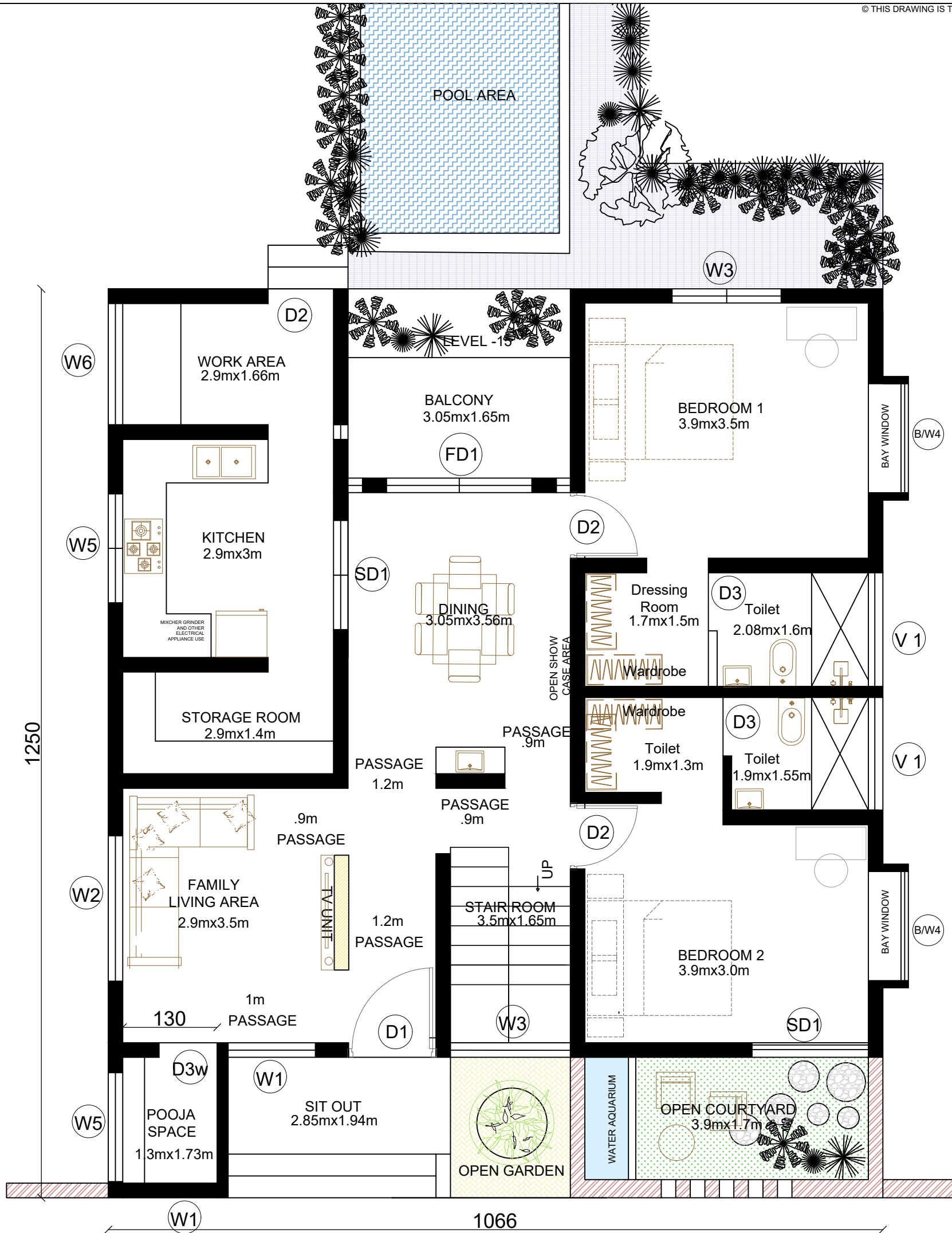
GROUND FLOOR PLAN AREA -1310 Sqr ft
