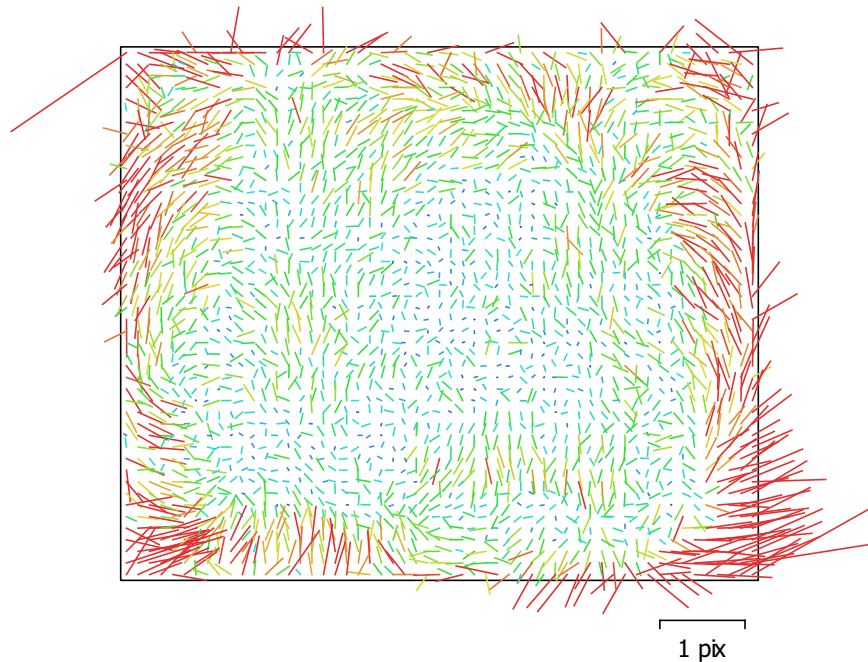
Fig. 2. Image residuals for BFS-PGE-50S5C-C.
