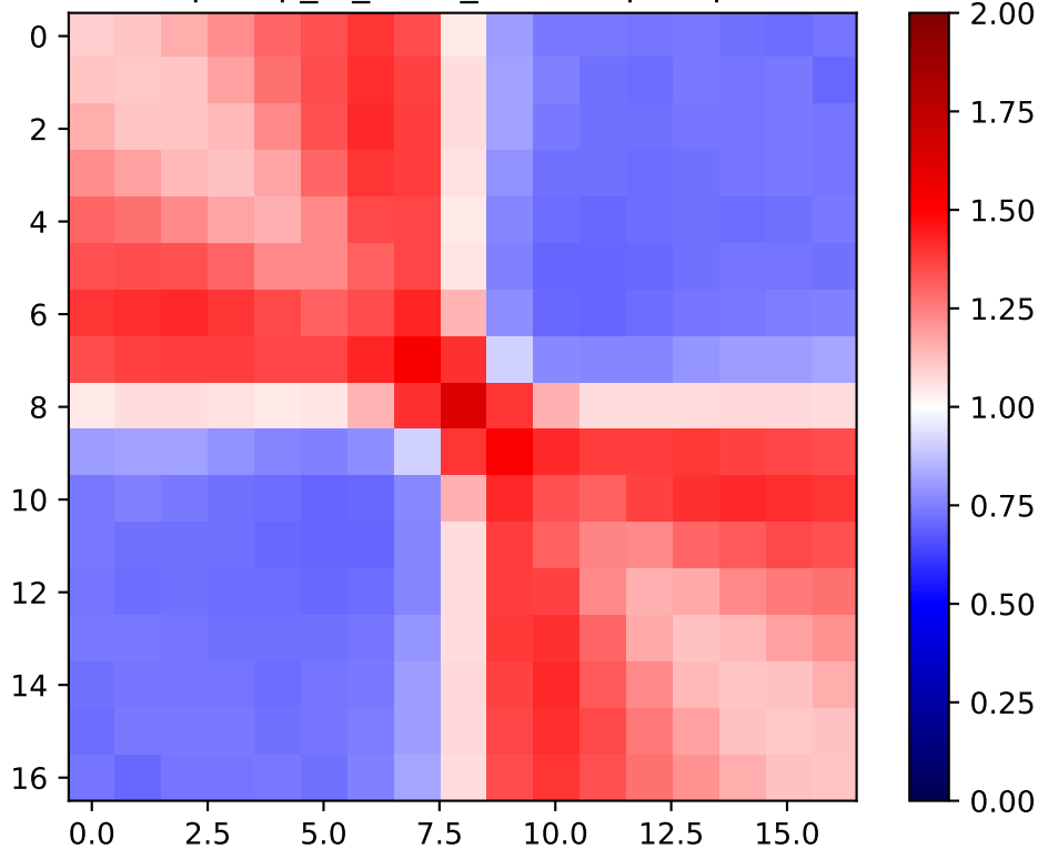
pileup_of_4654_borders pileup
