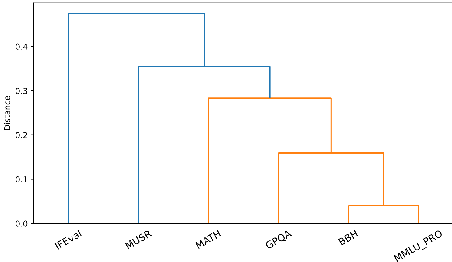
Benchmark clustering (linkage=average, distance=1-correlation)
