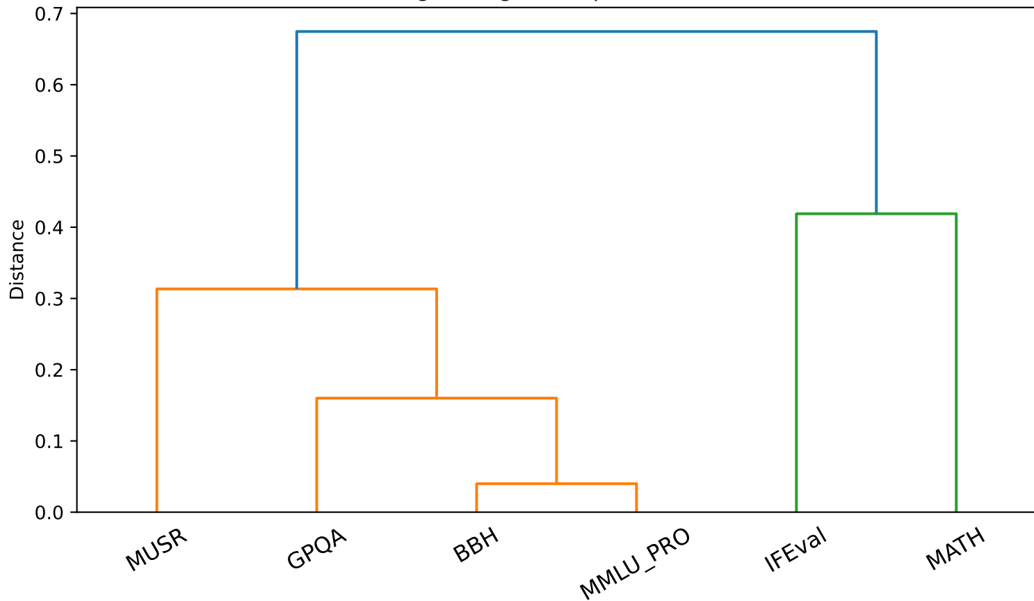
Benchmark clustering (linkage=complete, distance=1-correlation)
