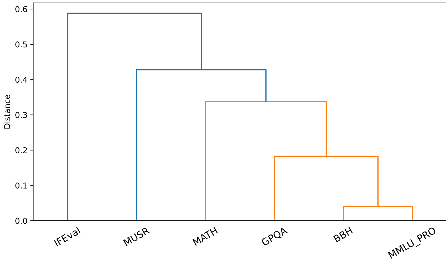
Benchmark clustering (linkage=ward, distance=1-correlation)
