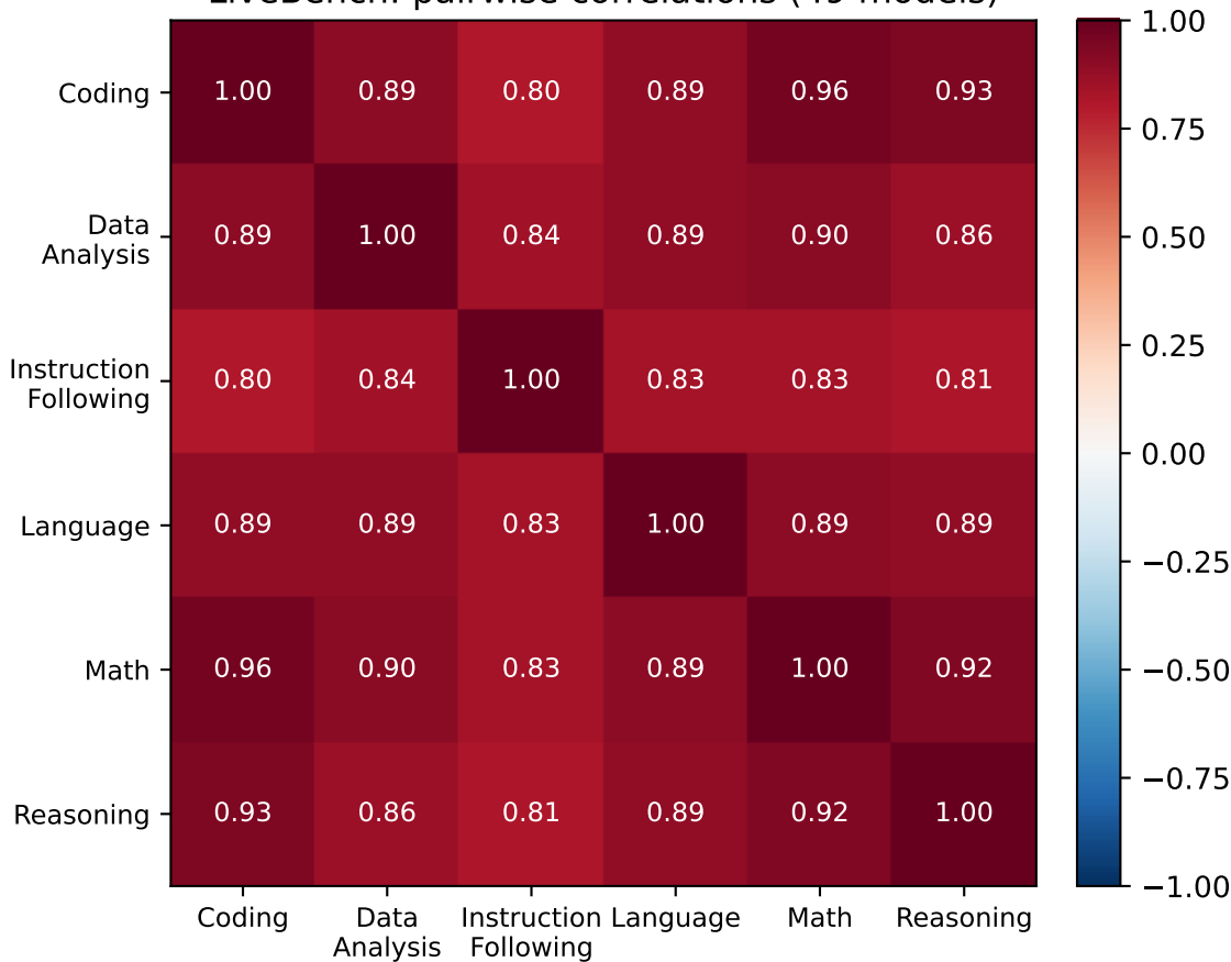
LiveBench: pairwise correlations (49 models)
