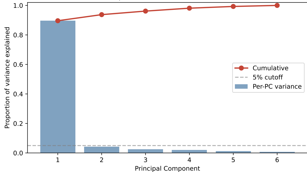
Scree plot: LiveBench (49 models, 6 categories) Spectral effective rank: 1.62
