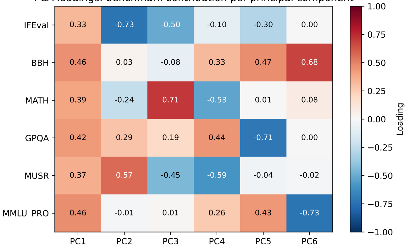
PCA loadings: benchmark contribution per principal component
