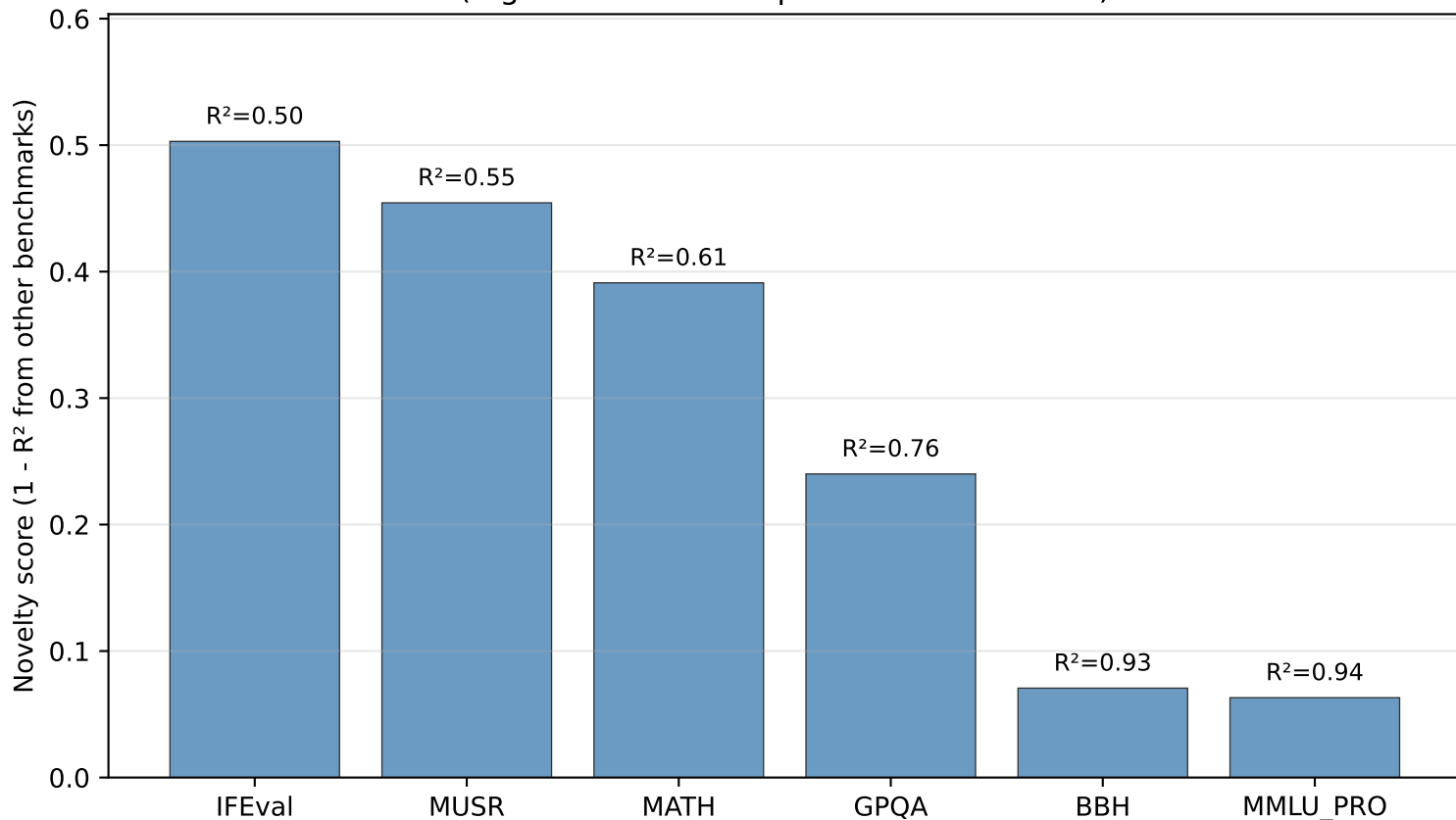
How much unique signal does each benchmark contribute? (higher = more independent information)
