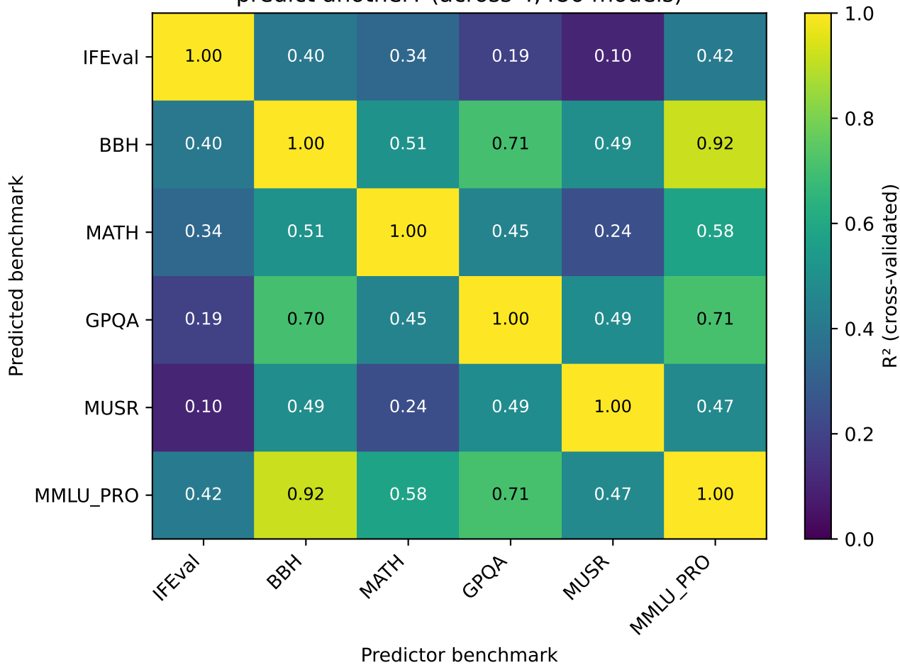
Pairwise predictive power: how well does one benchmark predict another? (across 4,486 models)
