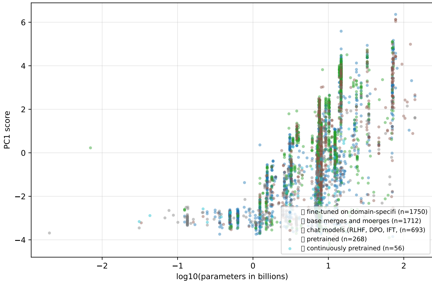
PC1 vs model size (Pearson r = 0.657 , n = 4,486 )
