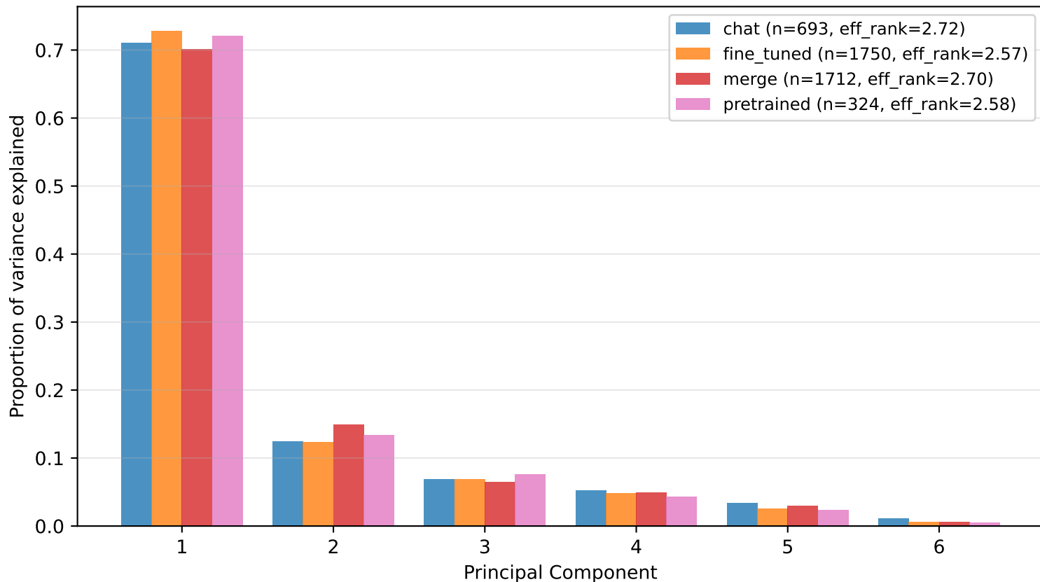
Explained variance by model category Effective rank is similar across categories
