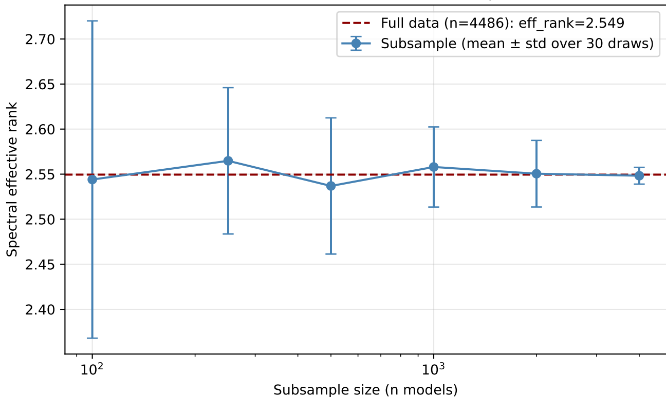
Effective rank is stable across subsample sizes
