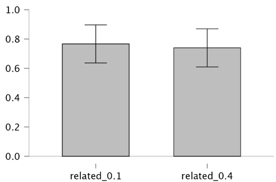
related_0.1 - related_0.4
