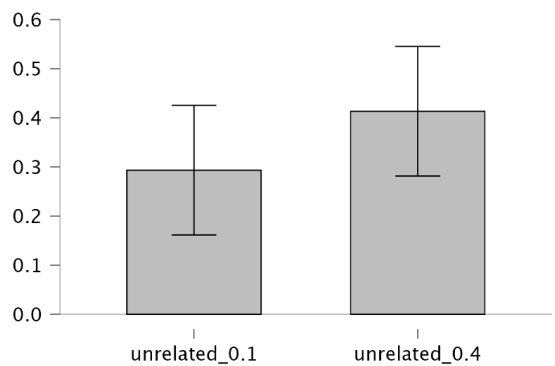
unrelated_0.1 - unrelated_0.4
