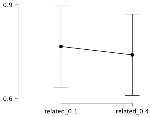
related_0.1 - related_0.4
