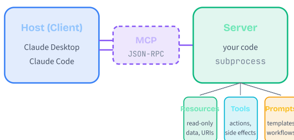
MCP Architecture
