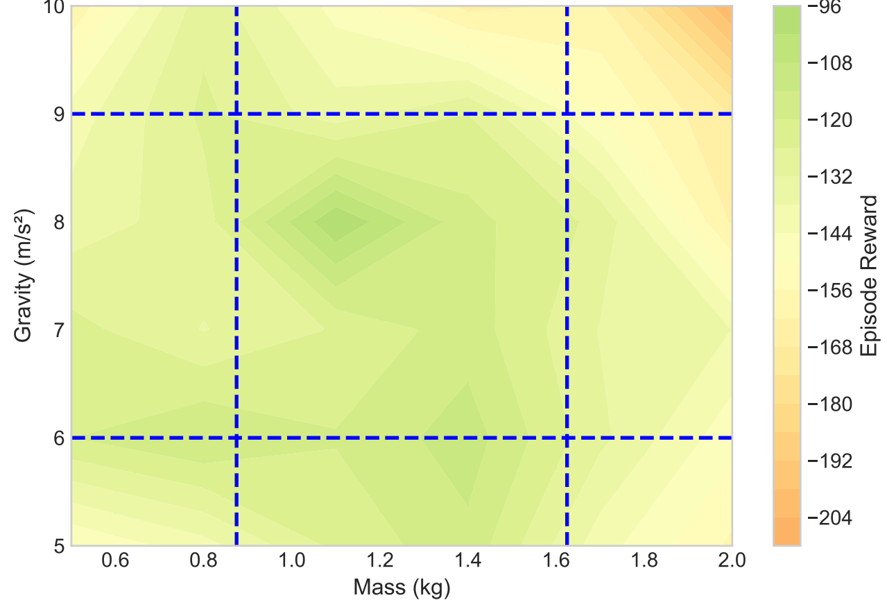
(b) Performance Contours
