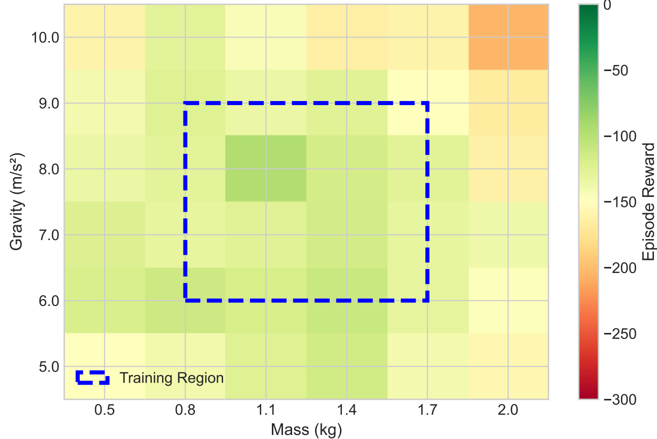
(a) Zero-Shot Performance in 2D Context Space
