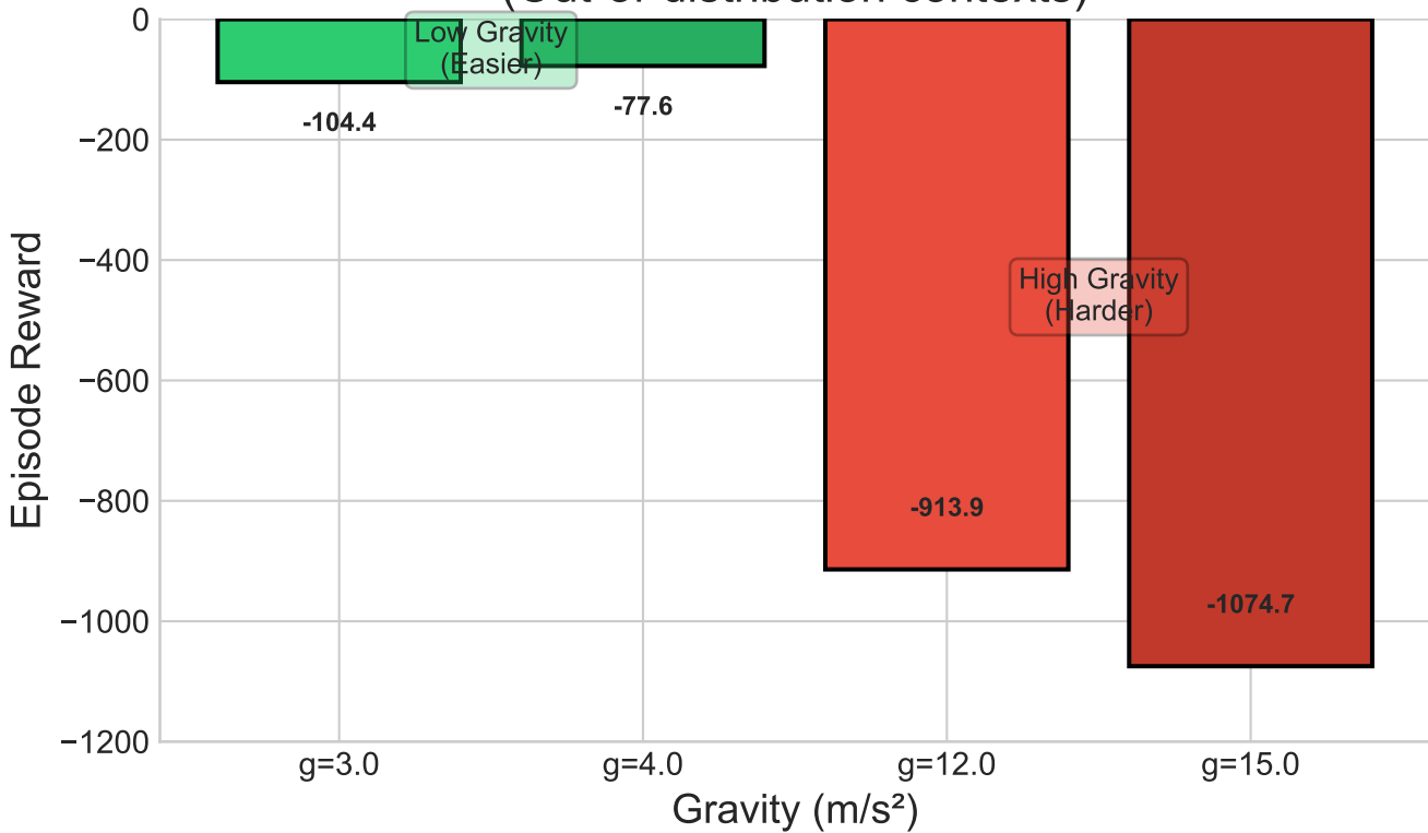
(b) Extrapolation Performance (Out-of-distribution contexts)
