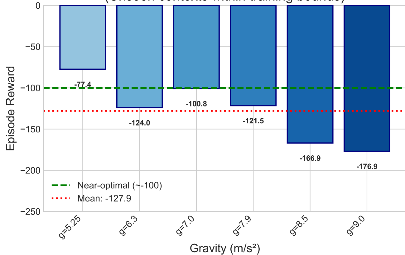
(a) Interpolation Performance (Unseen contexts within training bounds)
