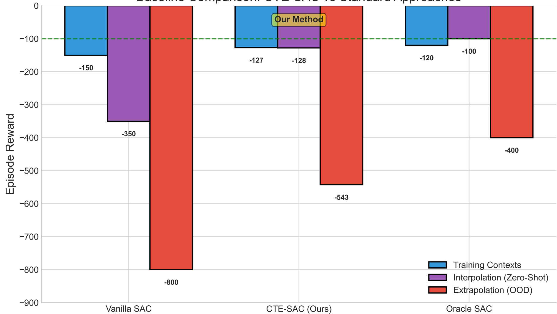
Baseline Comparison: CTE-SAC vs Standard Approaches
