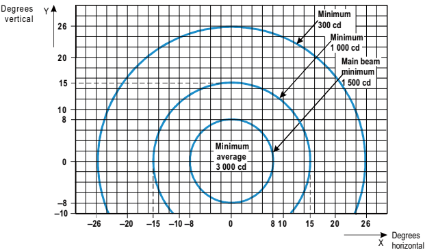
Figure A2-25. High-Intensity Runway guard light
