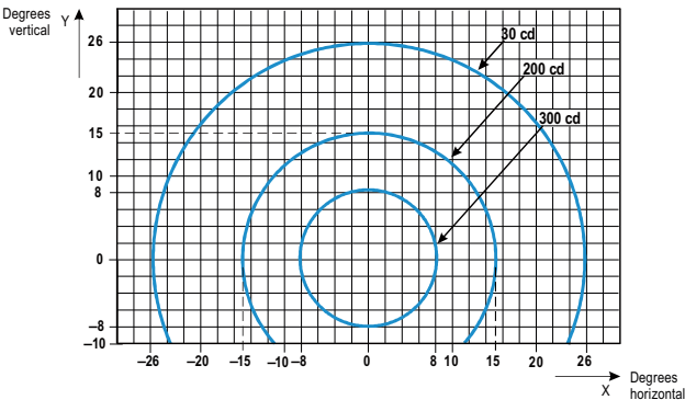
Figure A2-24. Low-Intensity Runway guard light
