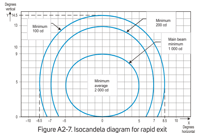
Figure A2-7. Isocandela diagram for rapid exit taxiway indicator light with 15 m longitudinal spacing (yellow light) for CAT III
