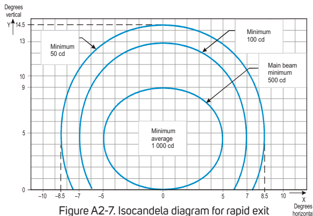
Figure A2-7. Isocandela diagram for rapid exit taxiway indicator light with 15 m longitudinal spacing (yellow light) for CAT I & II
