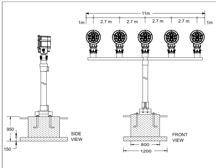
Elevated Installation
