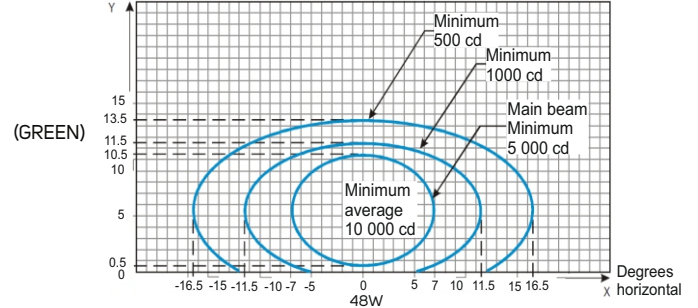
Threshold Wingbar Light
