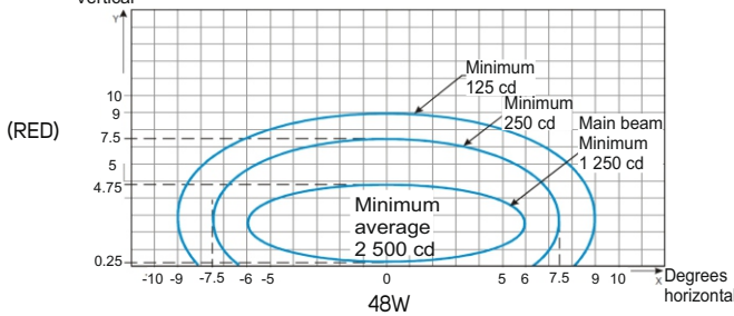
Runway End Light
