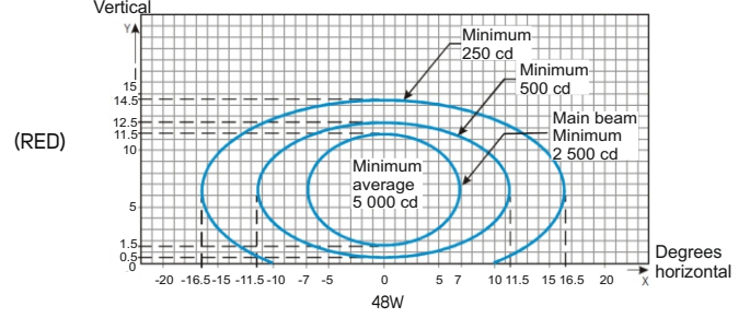
Approach Siderow Light
