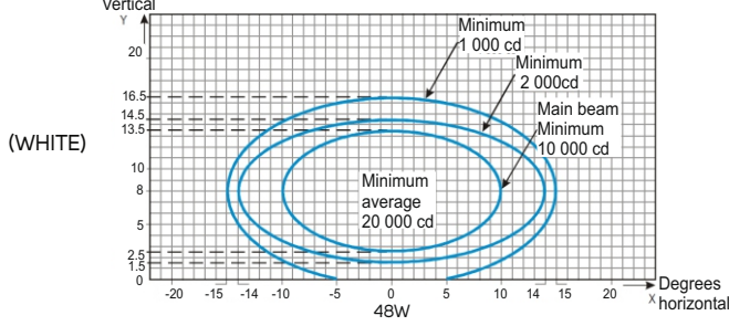
Approach Center & Crossbar Light
