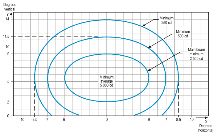
Runway Touchdown Zone Light ICAO Fig. A2-5
