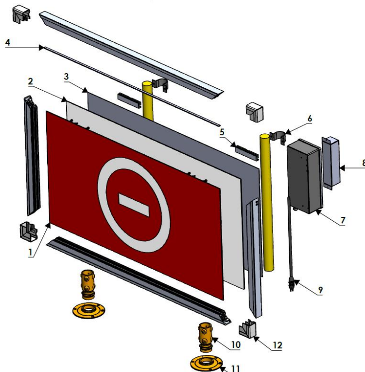
Exploded View
