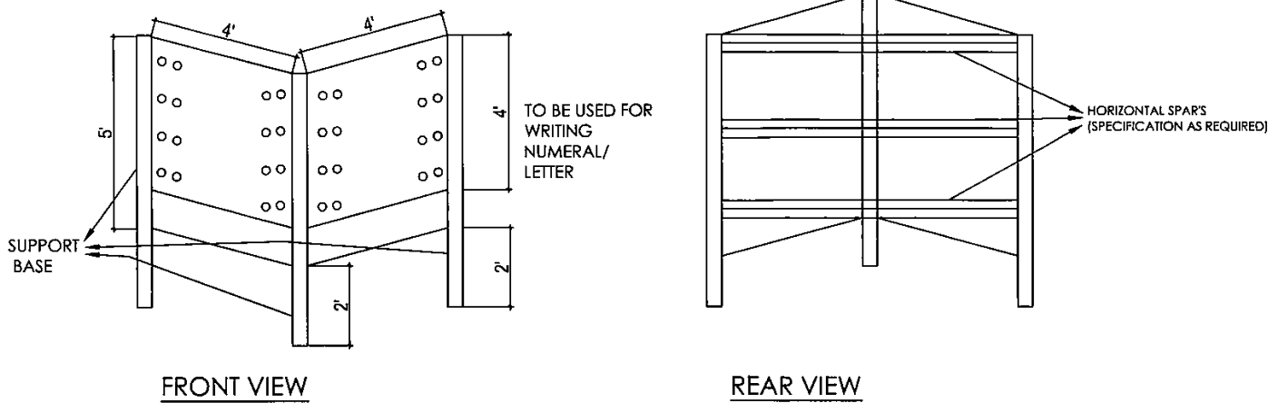
DETAIL OF DTGM BOARD
