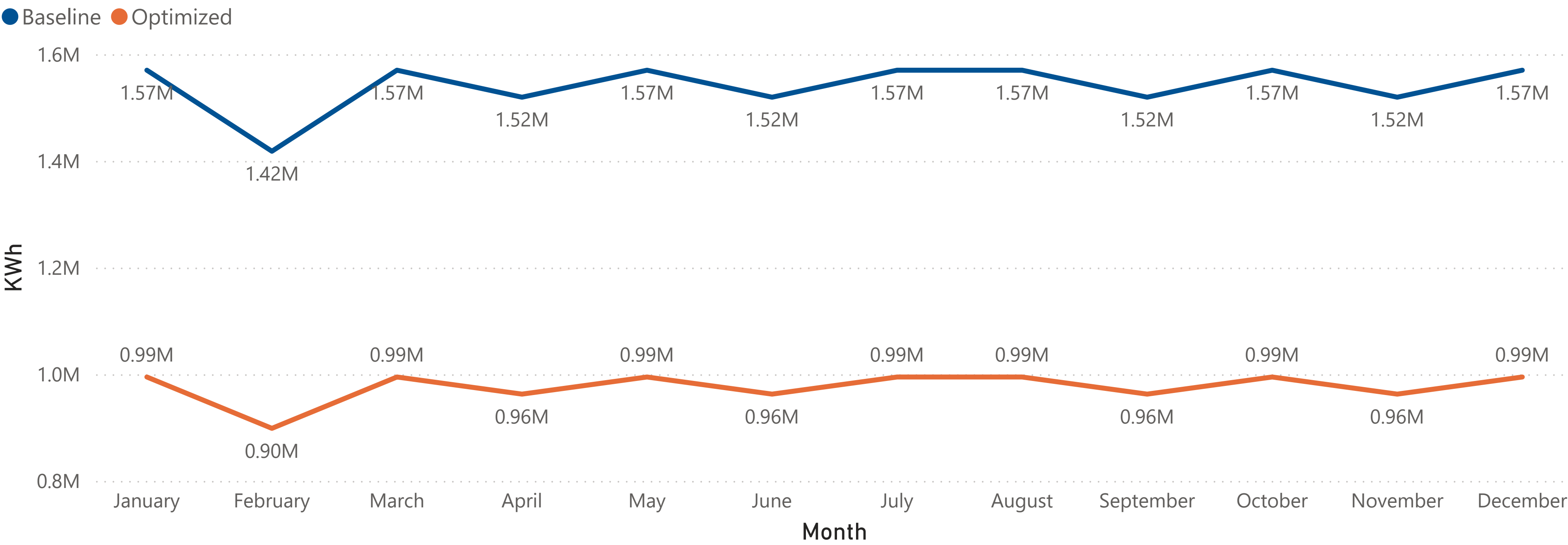
Fans Usage by Month
