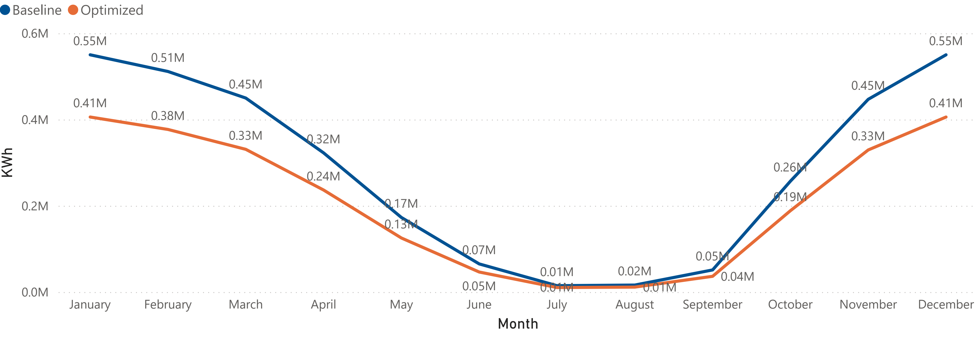
Heating Usage by Month
