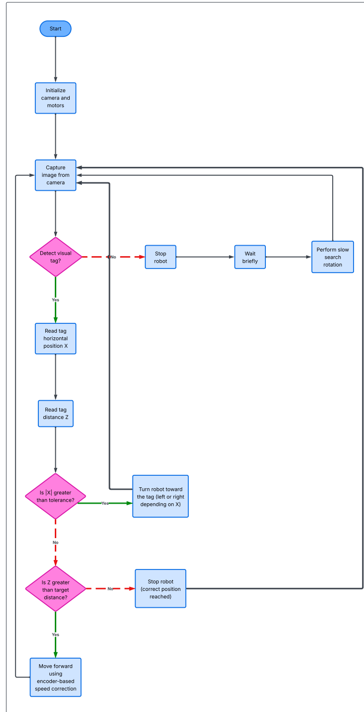
Mobile Robot "Follow-Me" Mission Flowchart
