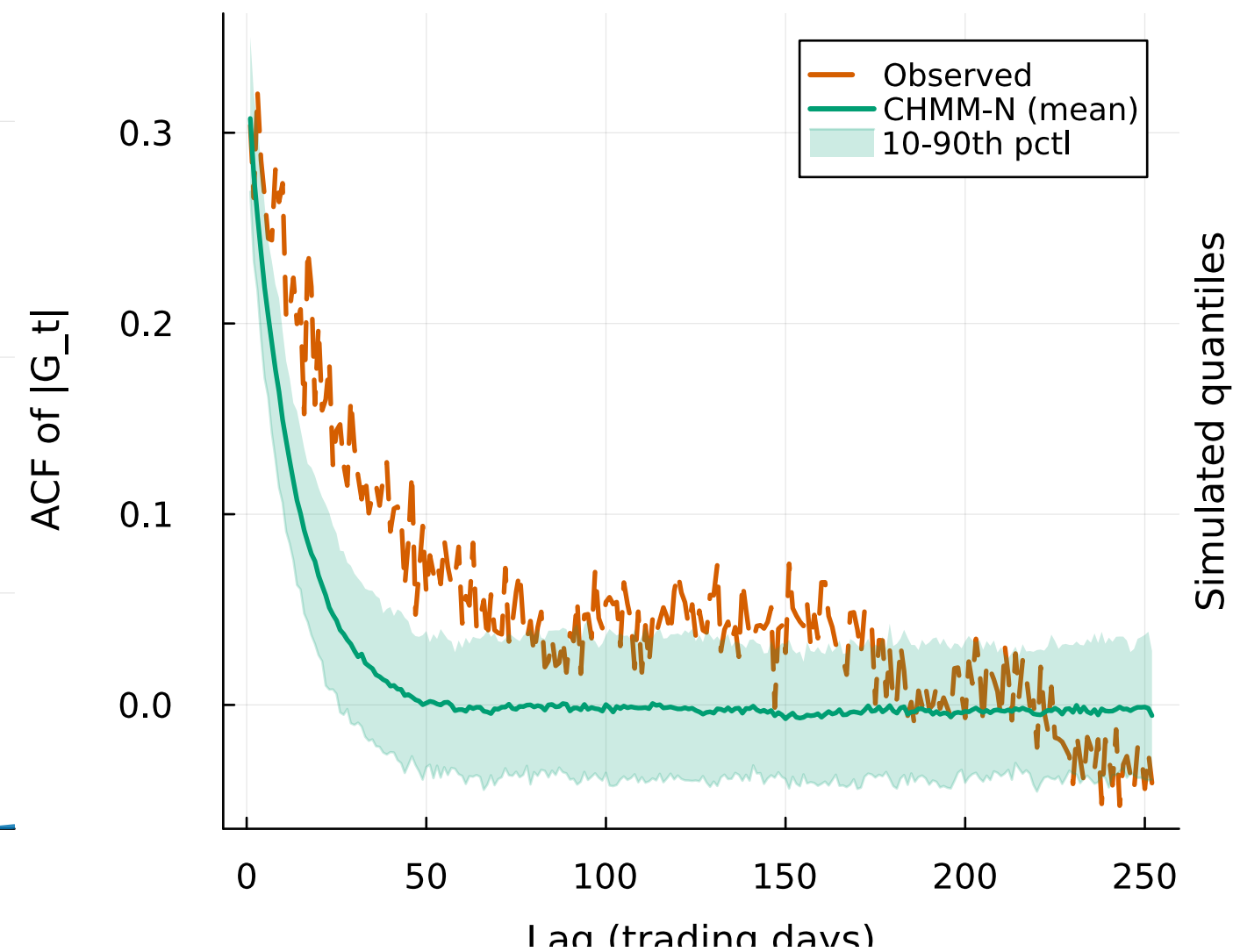
(b) ACF of |G_t|
