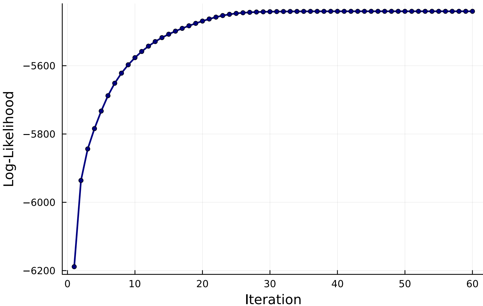
Baum-Welch Convergence (SPY, K=3)
