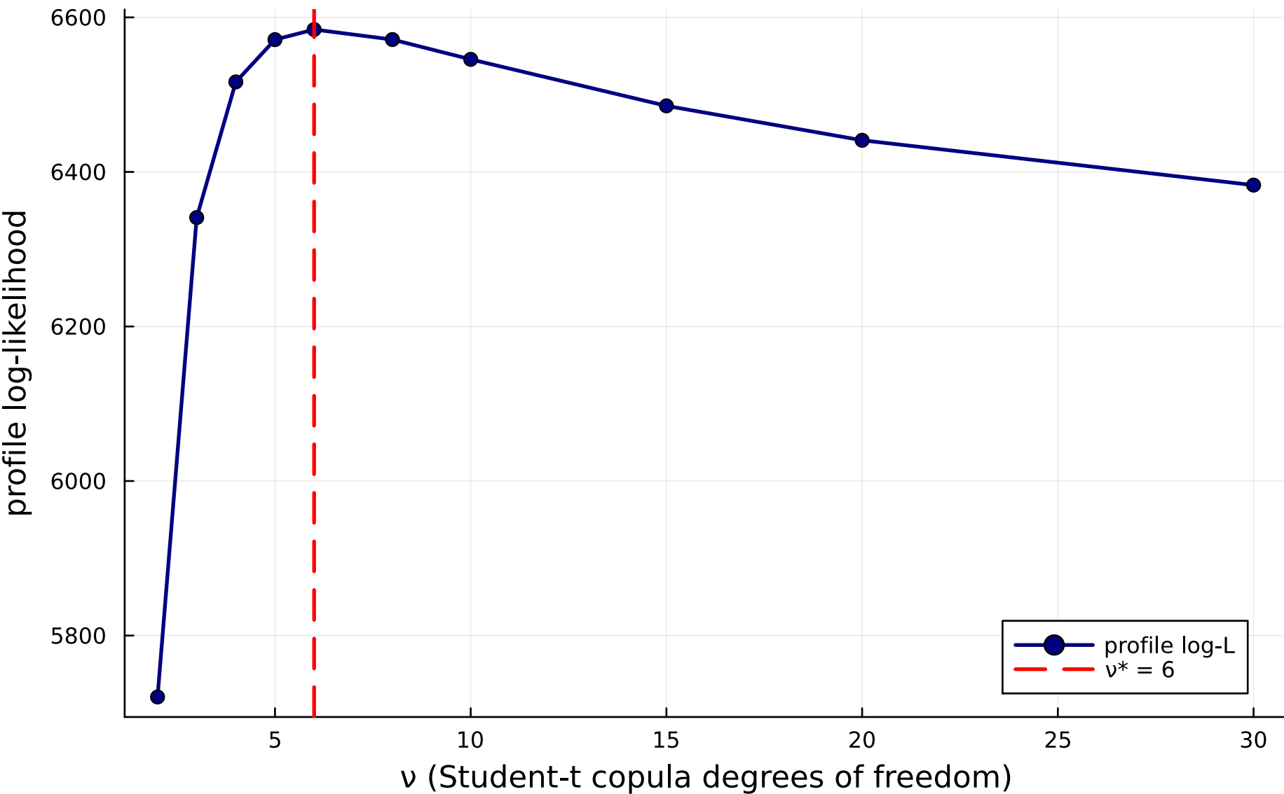
Student-t copula profile MLE — six-asset SPY cross-section
