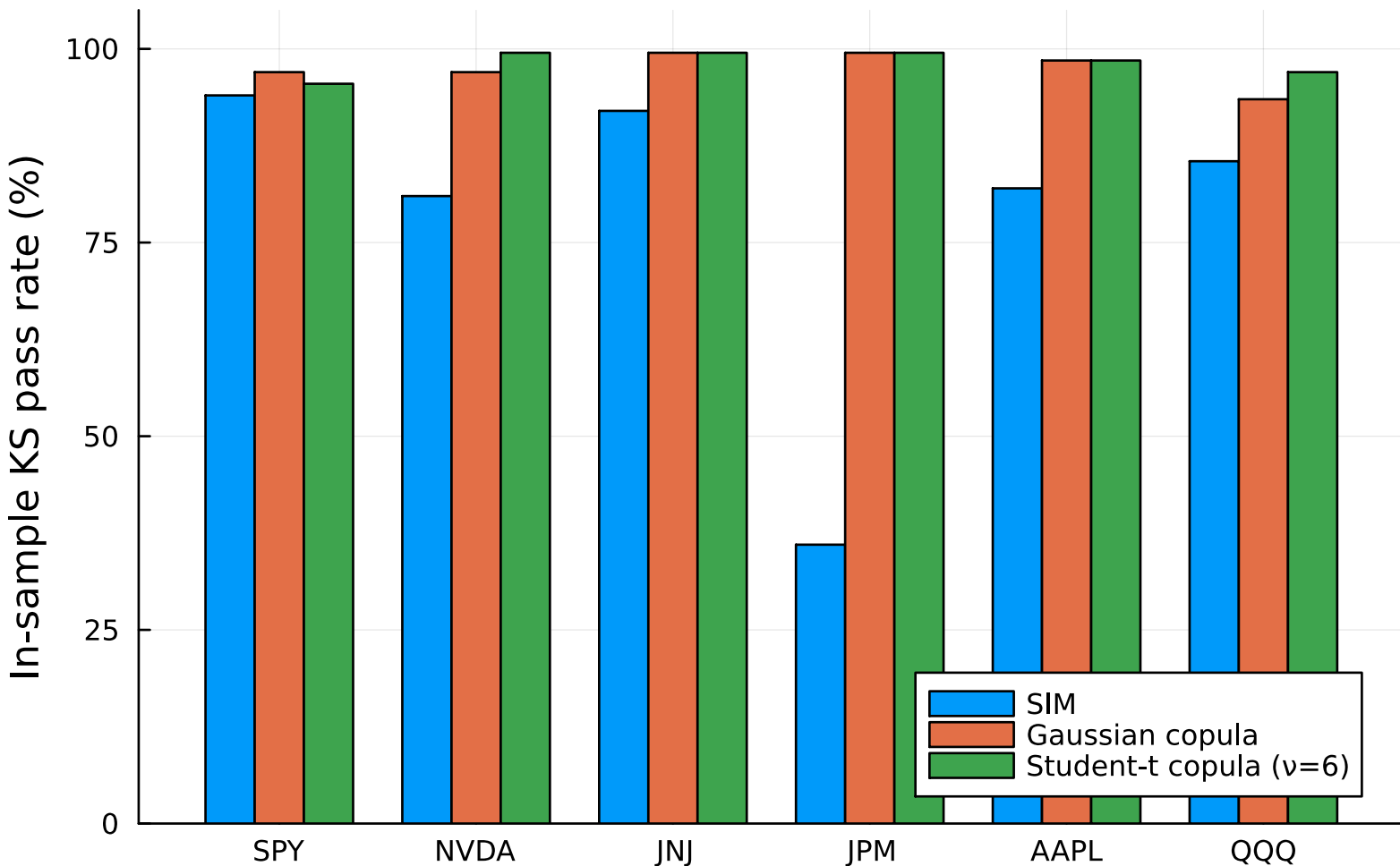
Per-asset in-sample KS pass rates
