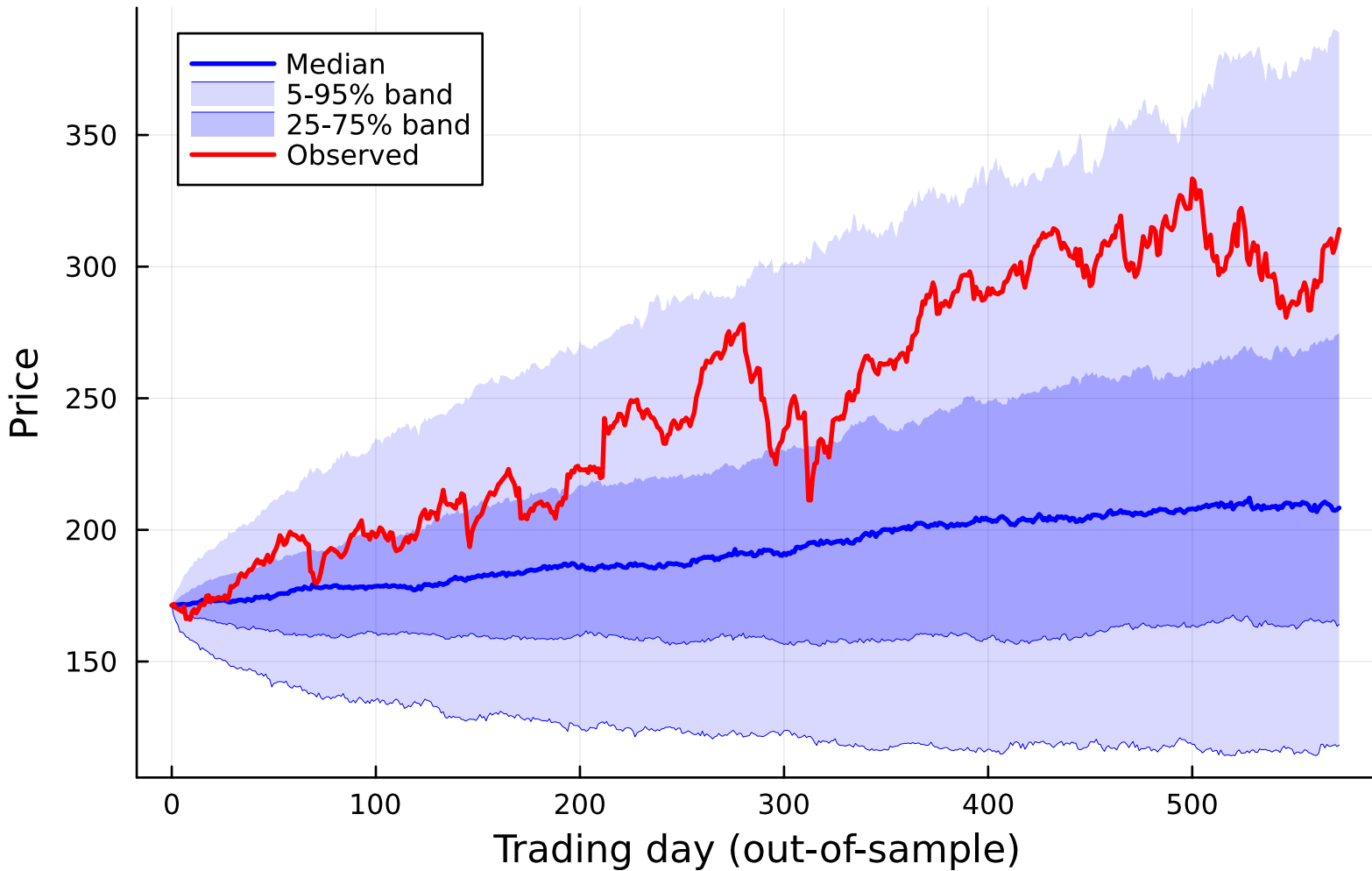
JPM - CHMM-L price fan (K=18, 500 paths)
