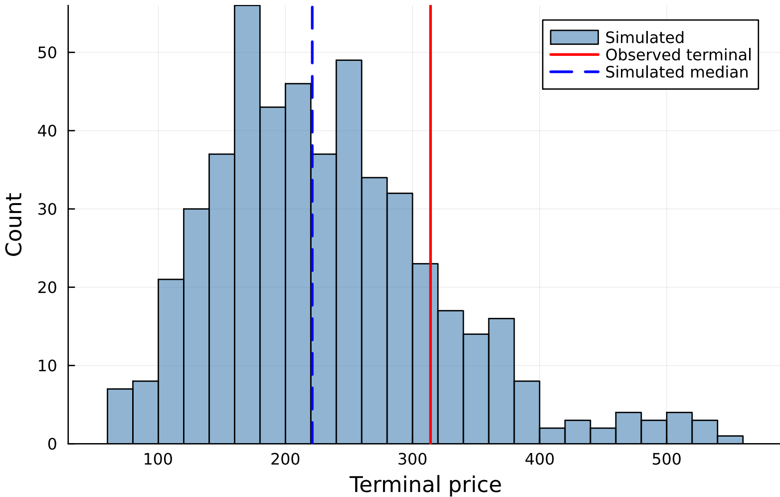
JPM - CHMM-N terminal price (n=500)
