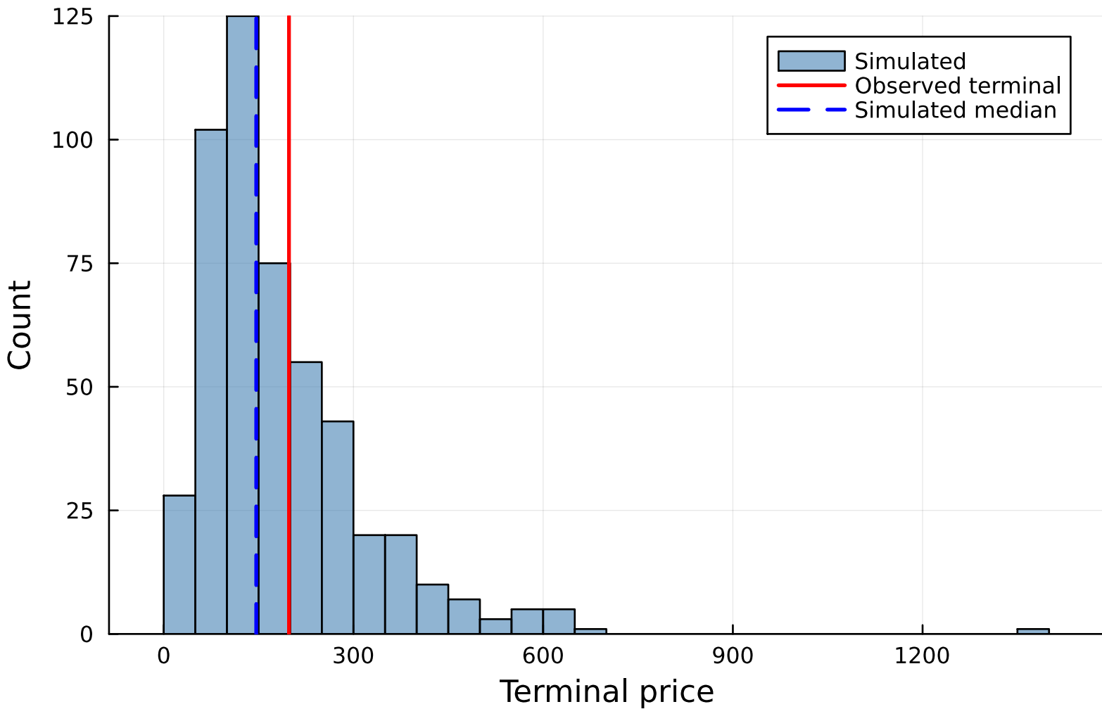
NVDA - CHMM-N terminal price (n=500)
