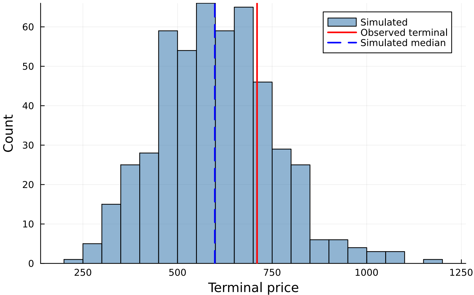
SPY - CHMM-N terminal price (n=500)
