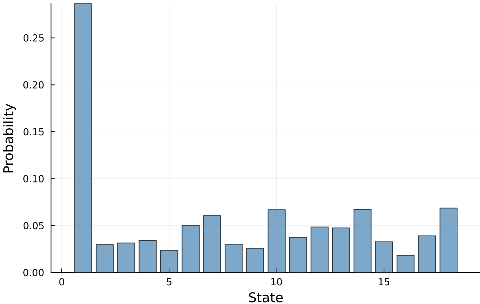
Stationary Distribution (CHMM-L, K=18)
