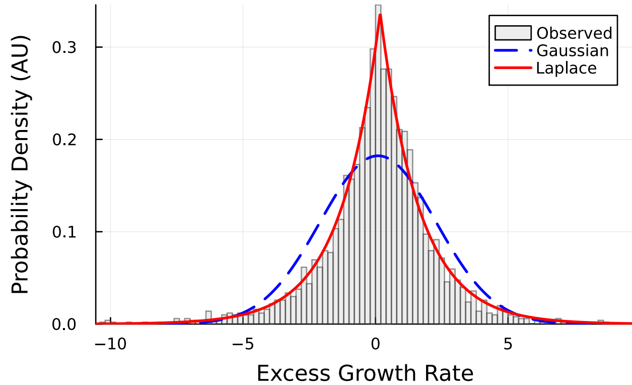
(a) Marginal Distribution
