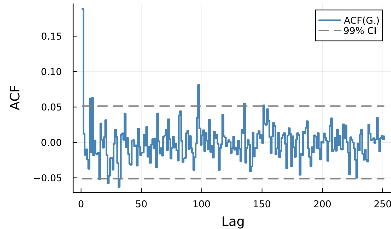
(c) Returns ACF
