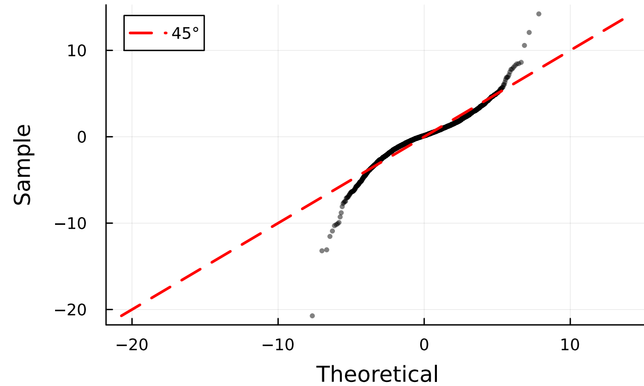
(b) Normal Q-Q Plot
