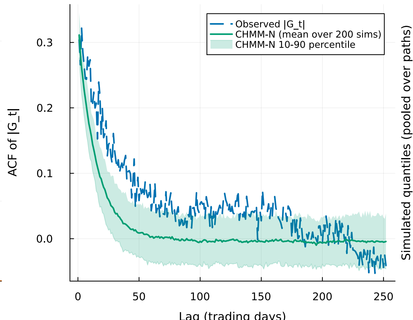
(b) ACF of |G_t| | lag 1..252 (trading days)
