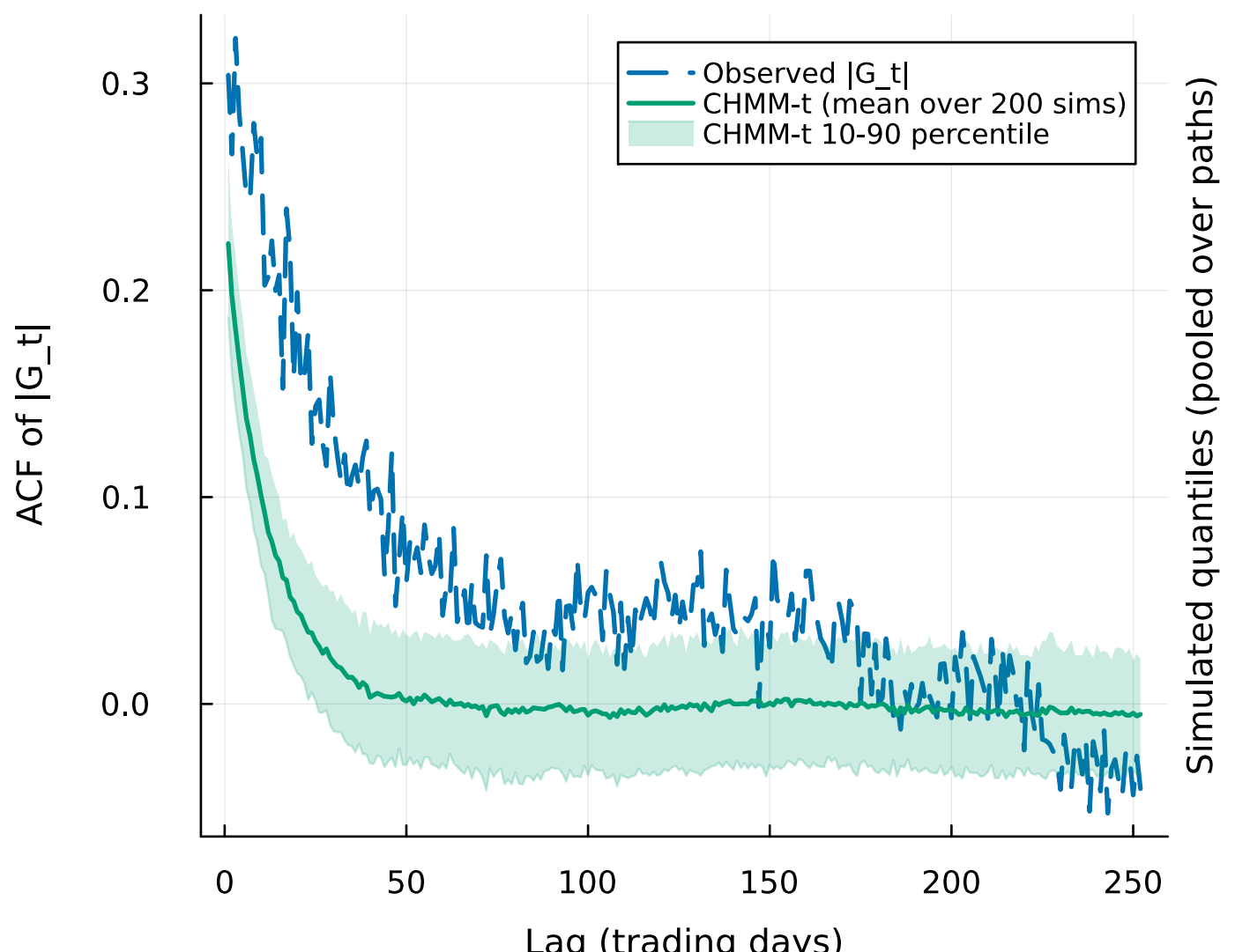
(b) ACF of |G_t| | lag 1..252 (trading days)
