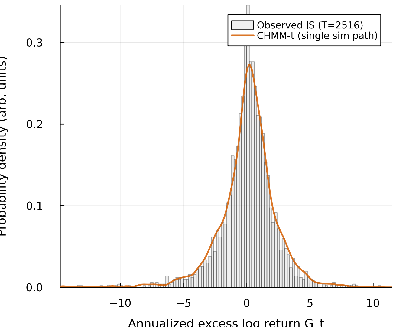
(a) IS return density | KS pass rate = 94.1% of 1000 paths at alpha=0.05
