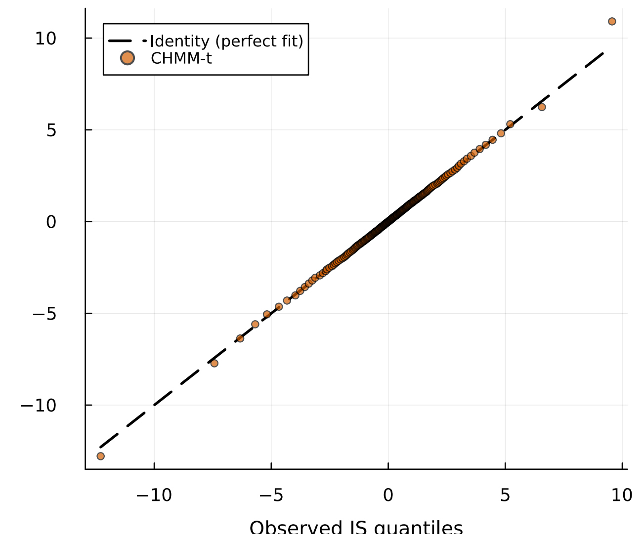
(c) Tail Q-Q plot | quantile grid 0.1% .. 99.9%
