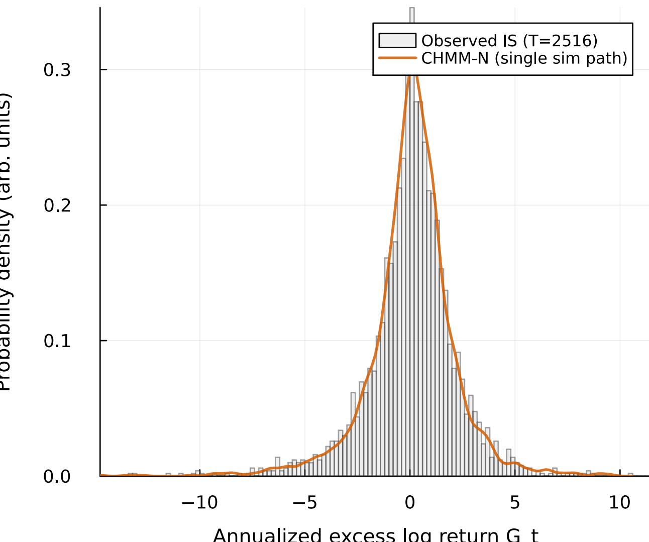
(a) IS return density | KS pass rate = 94.8% of 1000 paths at alpha=0.05
