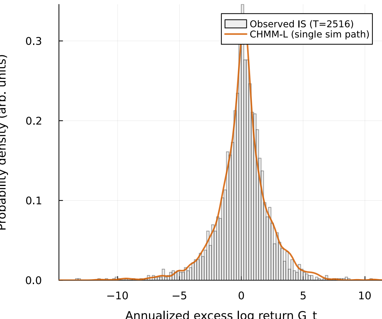
(a) IS return density | KS pass rate = 82.3% of 1000 paths at alpha=0.05
